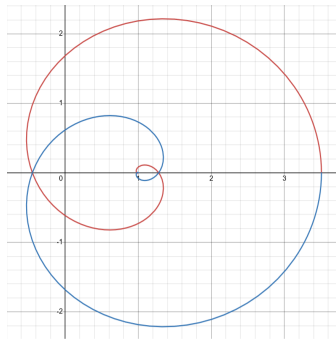
For z = 3, c = 1 .
