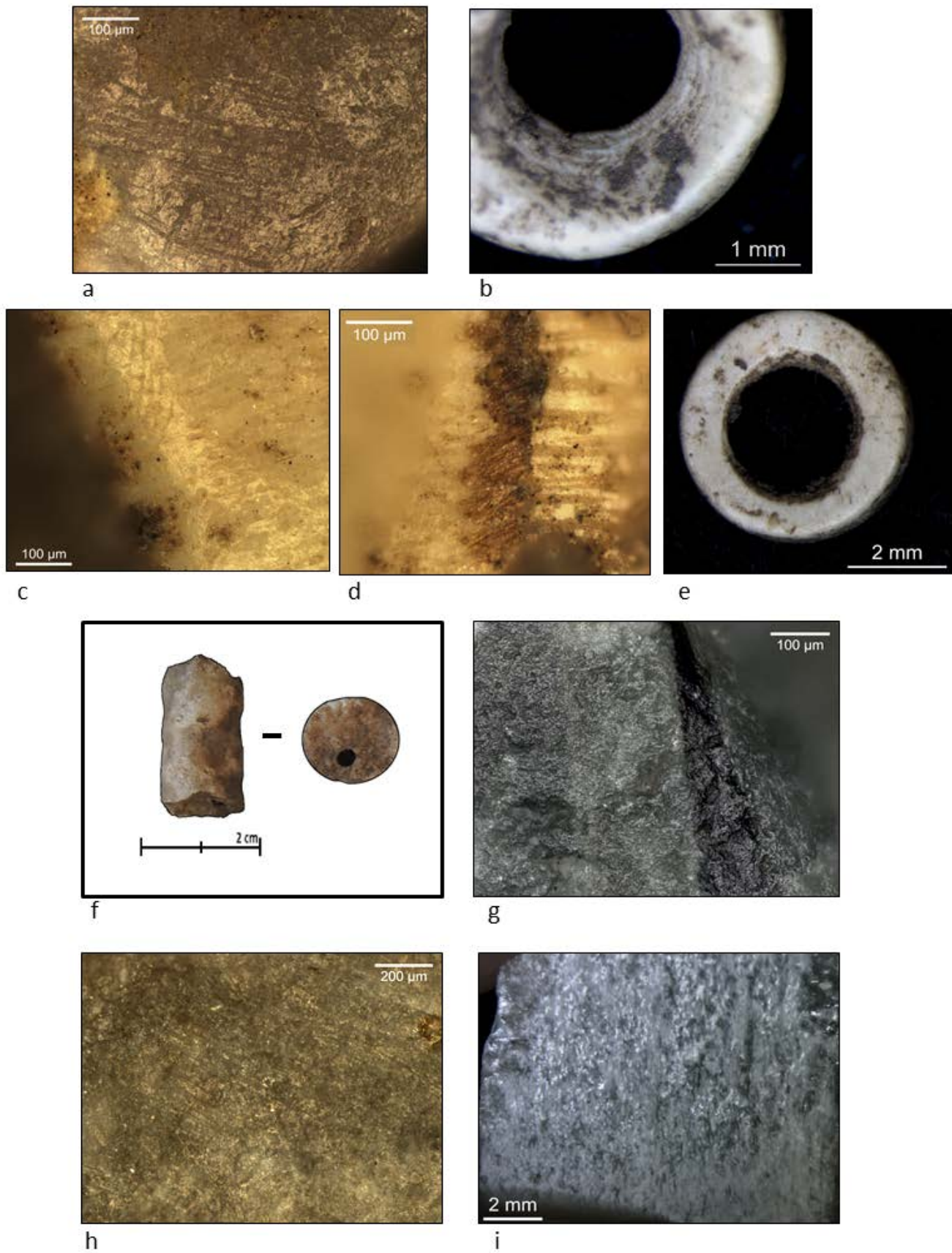
Figure 22: Manufacture and use-wear traces on shell beads (a–e). f: Calcite preform. Archaeological (g, h) and experimental grinding traces on lithic materials. g: diorite, h and i: calcite.
