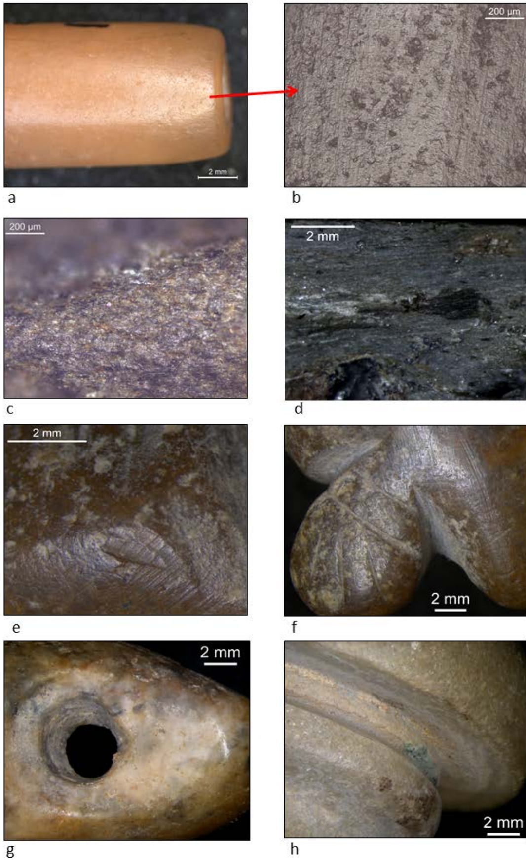
Figure 13: Grinding (a – c, f), scraping (e) and notching (f – h) on stone ornaments. Grinding experiment on mica-schist (d).
