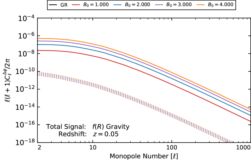
Figure 6.2: The purely C_\ell^{\Delta\varphi} luminosity distance power spectrum for f(R) gravity at a redshift z = 0.05 for various Compton wavelengths B_0 . The dotted curve denotes dark energy clustering (or anisotropic stress), zero for GR since M_{\text{Pl}} is a constant in the theory.
