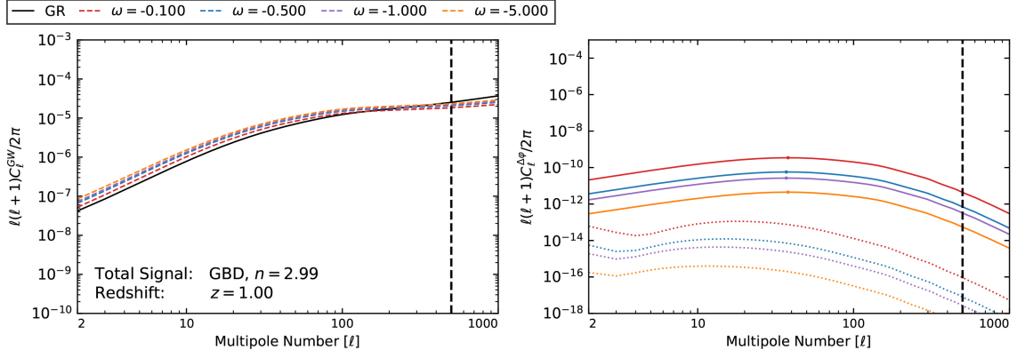
Figure P.3: Left: The C_l^{\text{GW}} luminosity distance power spectrum for GBD models varying \omega at redshift z = 1.00 for fixed n = 2.990 . Right: The resulting C_l^{\Delta\varphi} luminosity distance power spectrum for the same models at the same redshift.
