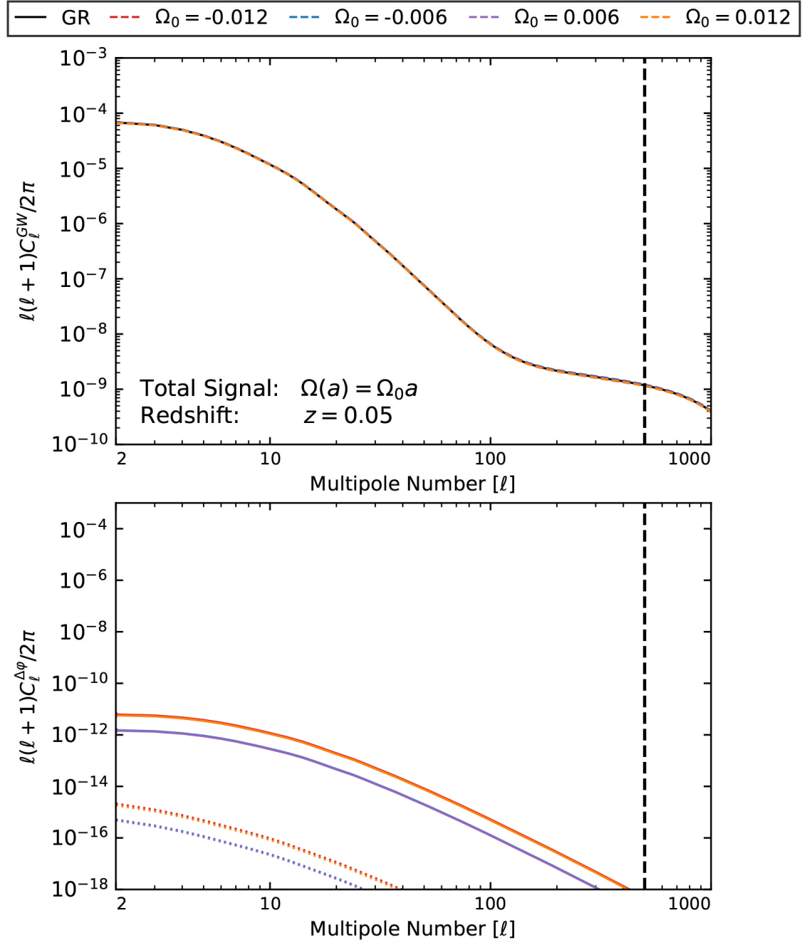
Figure 8.3: Top: The C_\ell^{\text{GW}} luminosity distance power spectrum for various \Omega_0 values following a linear relation. Bottom: The subsequent C_\ell^{\Delta\phi} luminosity distance power spectrum for the same models with the dotted lines representing dark energy clustering.
