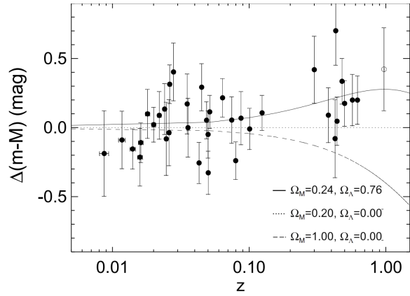
Figure 2.2: Figure from Riess et al. (1998) [23] in which they measured distances to distant Supernovae and tracked their redshift. As suggested from the plot and its legend, the best-fit model currently resides in one with a non-zero dark-energy composition.
