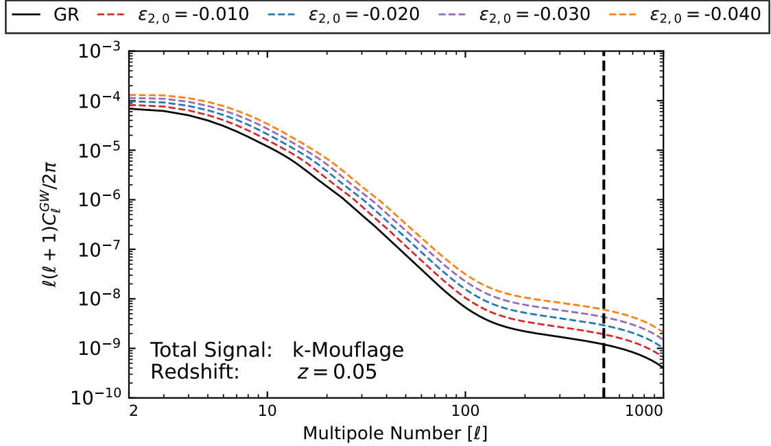
Figure 8.9: The C_\ell^{\text{GW}} luminosity distance power spectrum for k-Mouflage theories varying \varepsilon_{2,0} at redshift z = 0.05 .
