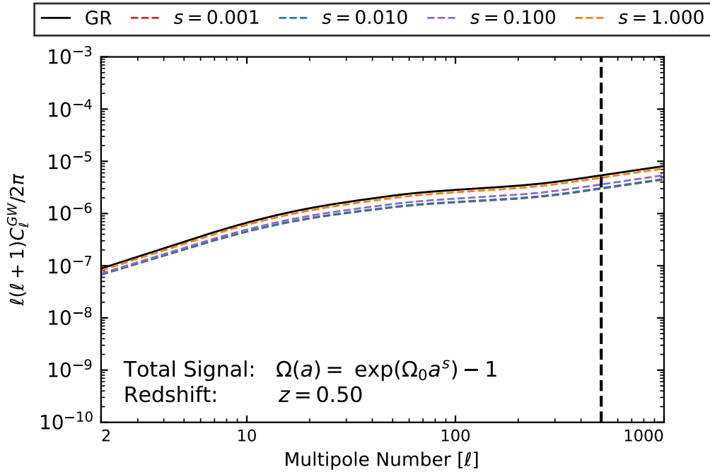
Figure N.2: The C_\ell^{GW} luminosity distance power spectrum for various exponential values where \Omega_0 follows an exponential relation. Redshift z = 0.50 .
