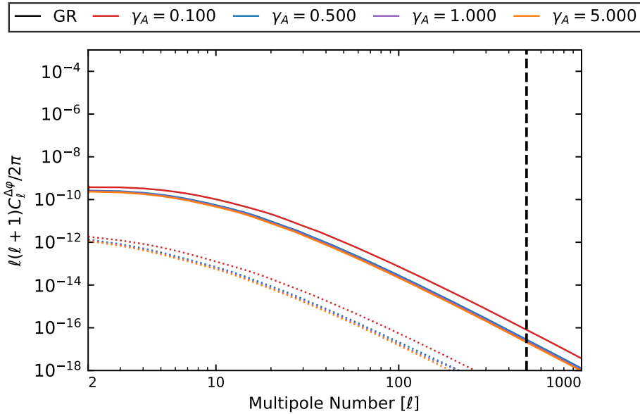
Figure 8.8: The C_\ell^{\Delta\phi} power spectrum for various k-Mouflage theories sampled at z = 0.05 . The dotted lines correspond to the dark energy clustering contribution of the theory.
