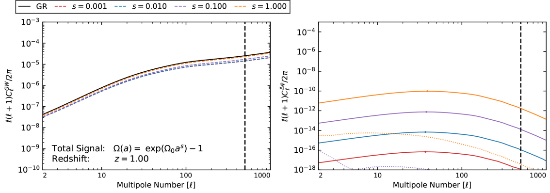
Figure N.1: Left: The C_\ell^{GW} luminosity distance power spectrum for various exponential values where \Omega_0 follows an exponential relation. Right: The C_\ell^{\Delta\varphi} luminosity distance power spectrum for the same models at the same redshift. Both plots are at a redshift z = 1.00
