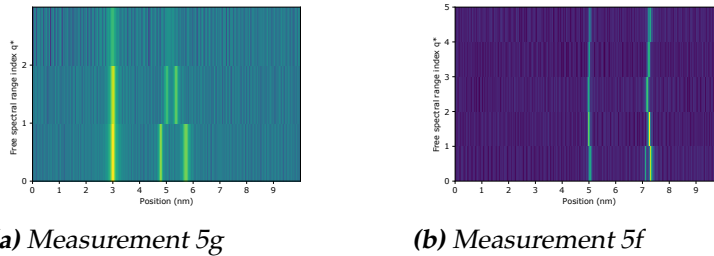
Figure 5.6: False color plots of N=1 modes of two measurements on a 5 \mu\text{m} cavity. Both measurements have a splitting on the right peak. But for higher q there are only two peaks. Also note how for higher q the positions of the two right peaks tends to converge to a position between the splitting for lower q .
