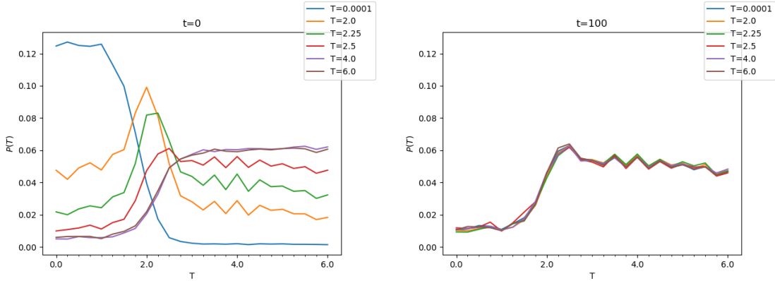
(a) The temperature probability distributions at the start of the RBM-flow.
