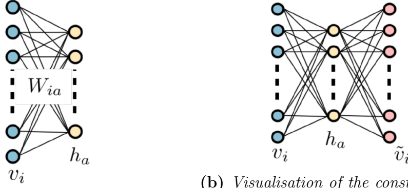
(a) Visualisation of the architecture of an RBM (b) Visualisation of the construction of a new configuration \tilde{v}_i from a configuration v_i .
