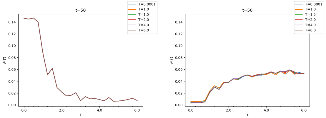
(a) RBM trained on T = 0 .
