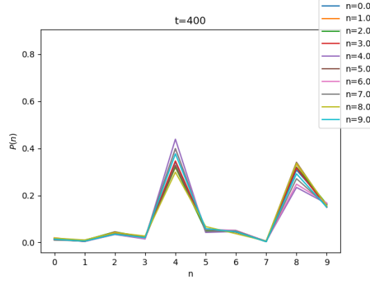
Figure 4.13: MNIST The end of the RBM-flow for an RBM trained at fours, eights and a mixture of fours and eights.
