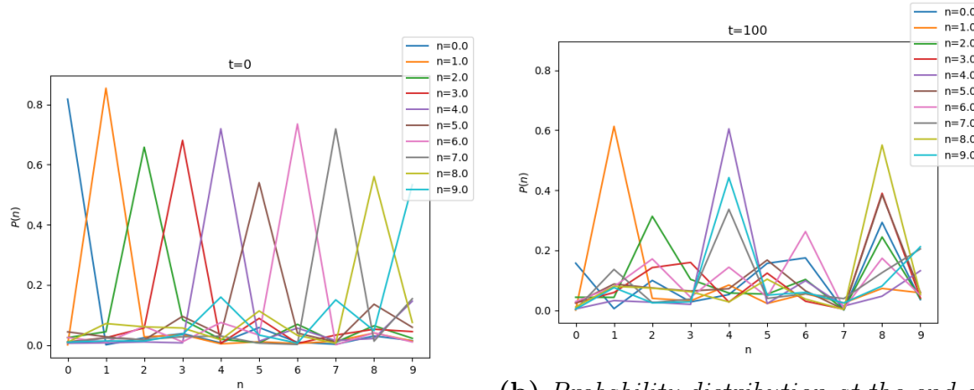
(b) Probability distribution at the end of the RBM-flow for an RBM trained on fours and eights.
