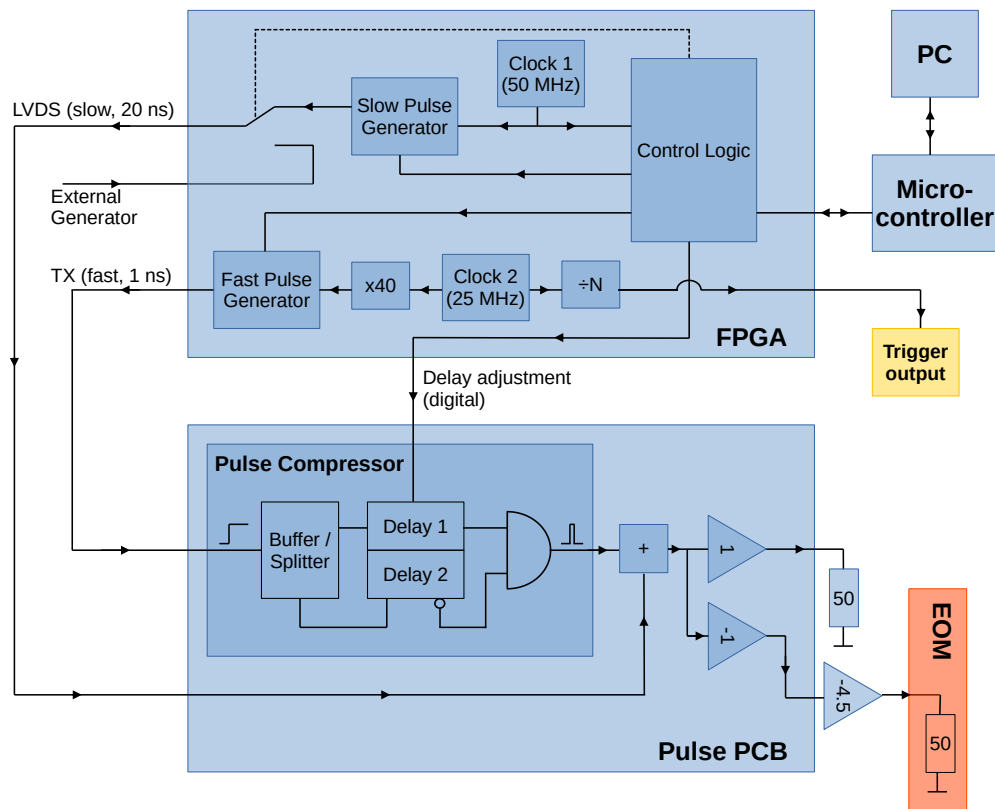
Figure 2.3: Schematic block diagram representing the pulser electronics. Long pulses are created by the FPGA at the desired frequency, which are then compressed to the desired lengths by the pulse compressor on the pulse PCB. Adapted from the Leiden university ELD.
