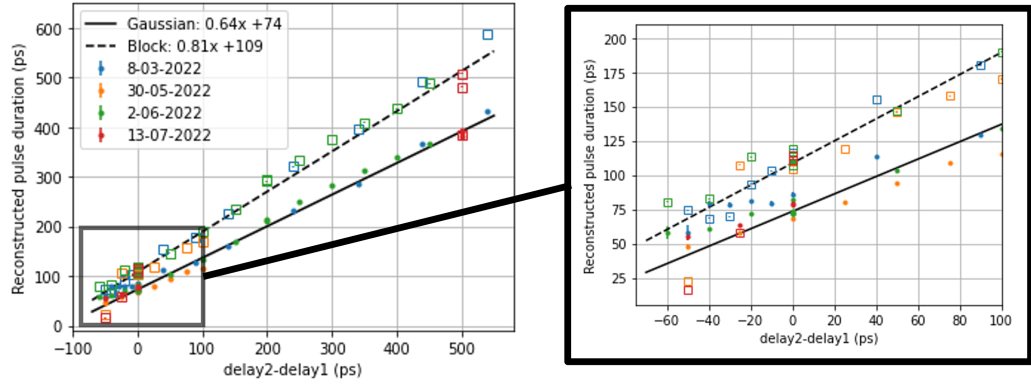
Figure 4.7: The reconstructed pulse durations for Gaussian pulse assumptions (circles) and block pulse assumptions (squares). The colors indicate data taken at different days. The solid black line indicates a linear fit through the Gaussian-ansatz data, and the dashed black line indicates a linear fit through the block-ansatz data. The figure on the right shows a zoomed-in plot of the short pulse region.
