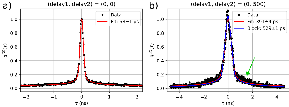
Figure 4.5: Measured g^{(2)}(\tau) for (a) a pulse with (delay1, delay2) = (0 ps, 0 ps) and (b) a pulse with (delay1, delay2) = (0 ps, 500 ps). The red lines show fits to the data assuming a Gaussian pulse. The blue line in (b) shows a fit assuming a block pulse.
