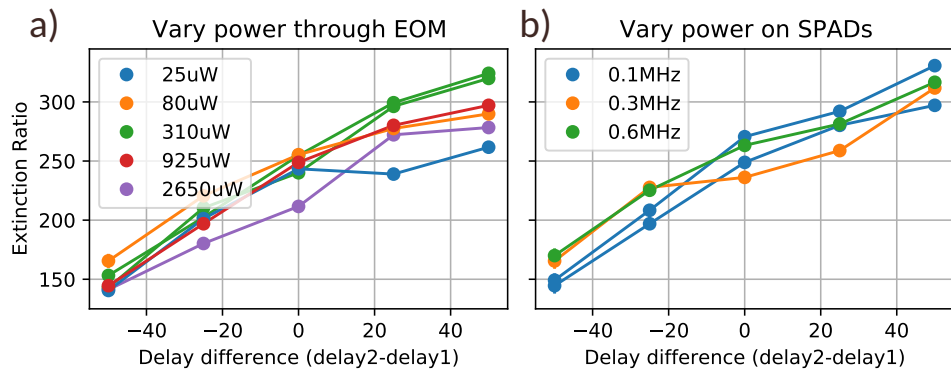
Figure 4.12: Reconstructed extinction ratios for different pulse durations. Figure (a) shows the extinction ratios for various different powers through the EOM (detector count rate 0.1 MHz), and (b) shows the extinction ratios for various powers on the detectors (EOM power 925 \mu W).
