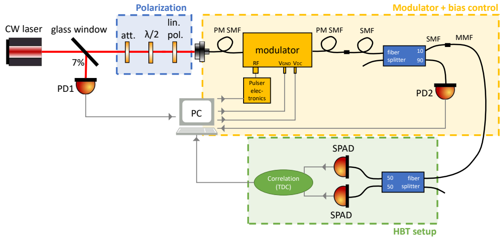
Figure 4.1: Schematic diagram of the experimental setup used to perform the HBT measurement of the laser pulses. The blue “Polarization” block shows components used to control the intensity and polarization of the light. The yellow “Modulator + bias control” block shows the EOM, pulser electronics, and the bias control setup. Finally the green “HBT setup” block shows the HBT part of the experiment.
