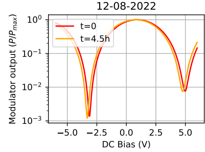
Figure 4.11: DC bias sweeps of EOM during power dependence measurements.
