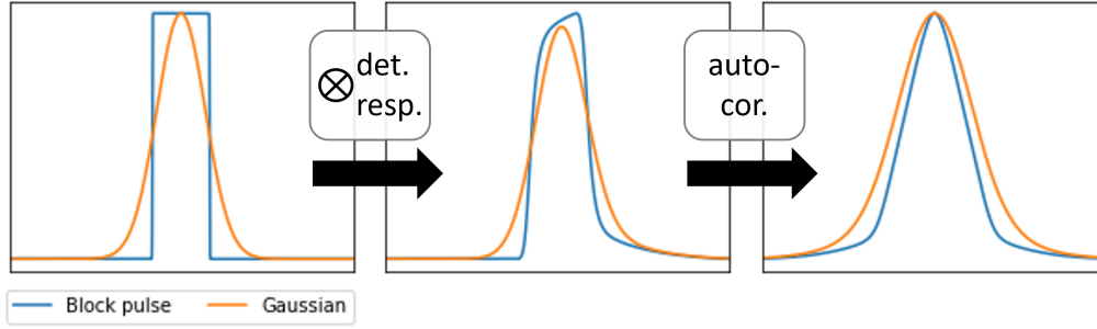
Figure 4.6: The difference in the model between a Gaussian (orange line) and block pulse (blue line) assumption, for long pulses. Shown is the original pulse, the convolution with detector response, and the autocorrelation. Both original pulses have a FWHM of 500 ps. The time axes of the three figures are equal.
