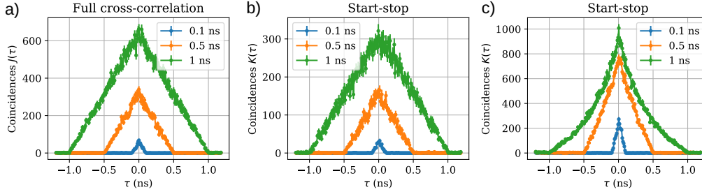
Figure 3.4: Simulation of full cross-correlation and start-stop operation for block pulses with perfect detectors and 0.1% background light. The pulses were simulated with three different pulse durations and a period of 100 ns. The pulses of (a) and (b) were simulated for 10 s with an intensity of 5 \cdot 10^7 photons/sec, and pulses of (c) were simulated for 10 ms with an intensity of 5 \cdot 10^9 photons/sec.
