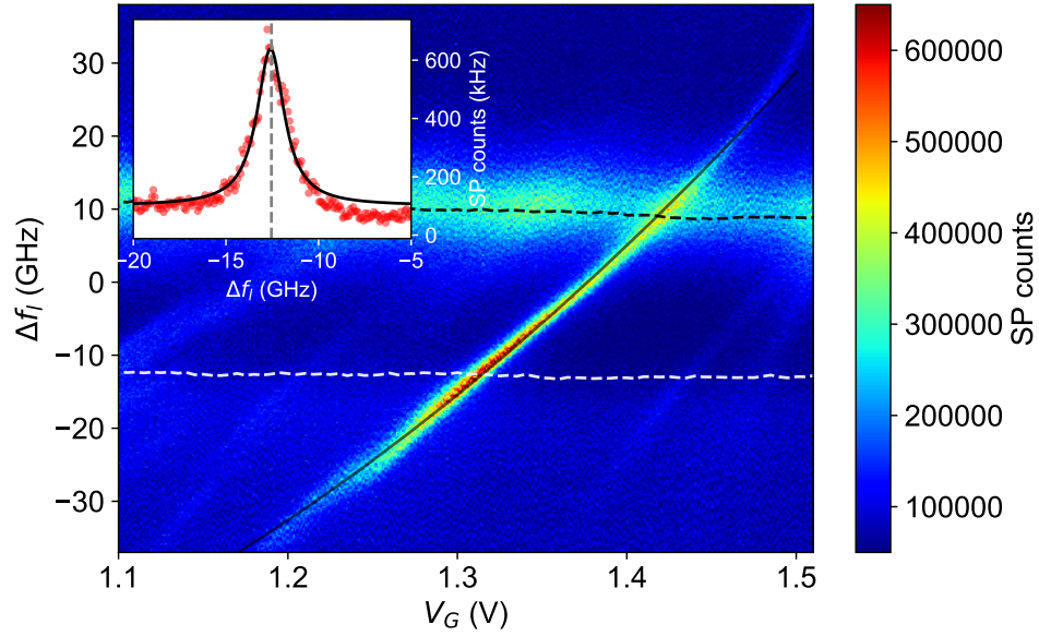
Figure 5.1: Voltage scan of a single quantum dot, measured in cross-polarization. The H- and V-modes are determined by Lorentzian fits of scans in co-polarization and are indicated here with a black and white dashed line, respectively. The inset shows a cross-section of the scan for a voltage of 1.31V.
