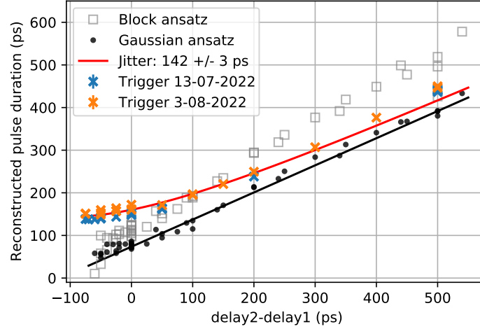
Figure 4.9: Reconstructed pulse durations for the TCSPC measurements. The black dots and grey squares show the results of the HBT measurements (Sec. 4.4.2) for a Gaussian and block pulse ansatz respectively. The red line through the trigger data shows a fit where a Gaussian jitter of 142 ps was added to the fit of the black line.
