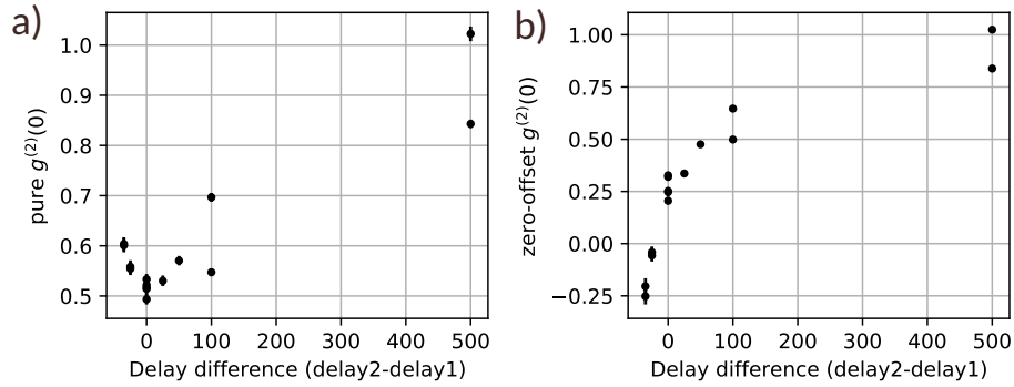
Figure 5.6: Measurements of g^{(2)}(0) for pulsed excitation, as function of the delay difference of the EOM electronics. Data taken on 21-07-2022. (a) shows the g^{(2)}(0) for peaks normalized to 1, (b) shows g^{(2)}(0) for offset subtracted and peaks normalized to 1.
