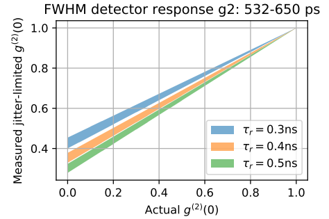
Figure 5.4: The maximally measured dip depths in CW g^{(2)}(\tau) versus the actual non-jitter-limited dip depths for detector jitters ranging from 532 ps to 650 ps, for three different lifetimes.
