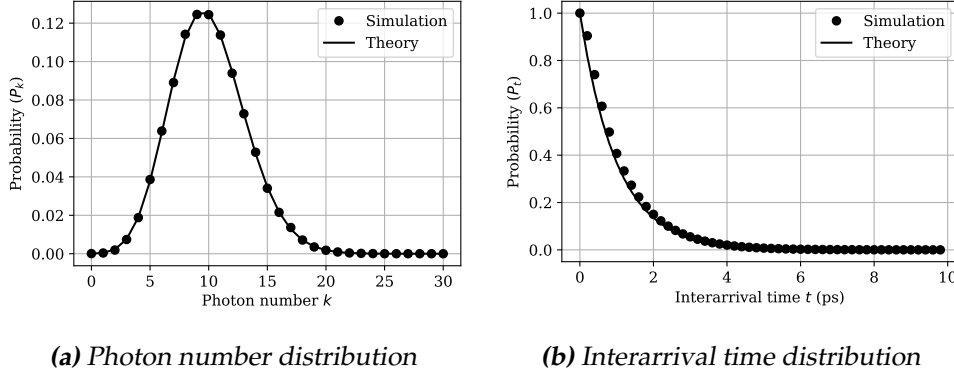
Figure 3.1: The Poissonian statistics of the simulated coherent light. This light stream consisted of 10^6 photons, with \Gamma = 10^{12} photons/sec and \Delta t = 1 fs. The dots represent the simulation and the solid line the theory from Equations 3.1 and 3.2. Figure (a) shows the photon number distribution for a counting time of 10 ps and (b) shows the interarrival time distribution.
