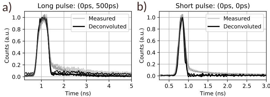
Figure 4.10: Deconvoluted TCSPC measurements. The grey lines show the original measurements and the black lines the deconvolutions with the detector response. Figure (a) shows a long pulse of \sim 520 ps and (b) a shorter pulse of \sim 160 ps.
