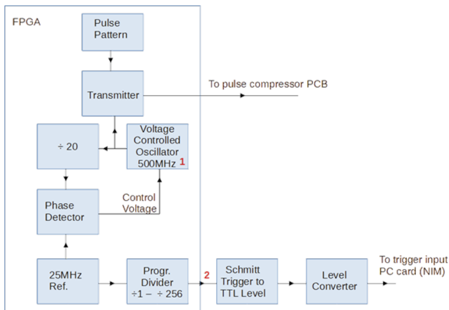
Figure II.1: A detailed schematic of the electronics surrounding the trigger pulse. The red 1 and 2 indicate possible sources of jitter. Figure provided by Harry Visser from the ELD.
