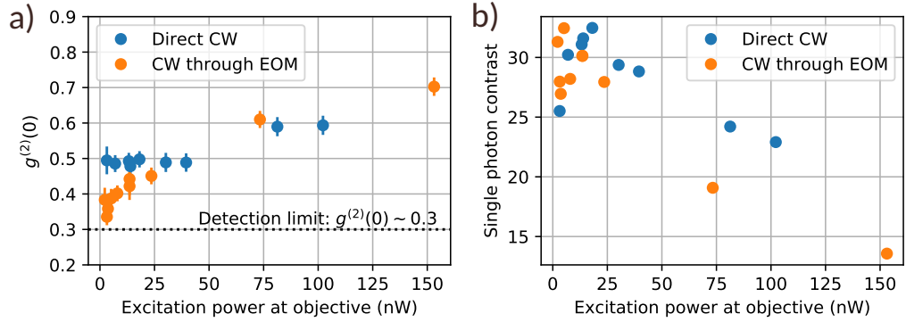
Figure 5.3: (a) Measurement of g^{(2)}(0) versus excitation power under CW excitation. (b) Single photon contrast versus excitation power. The blue dots were measured without the EOM in the setup, on 20-07-2022. The orange dots were measured through the EOM, operating at the maximum around V_{DC} = 0 , on 21-07-2022.
