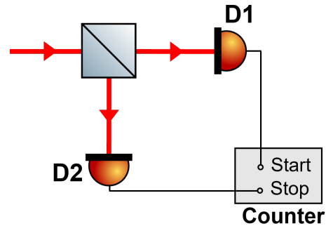
Figure 2.5: Schematic of a HBT setup using start-stop operation. The red arrows indicate the direction of the light and the orange half-circles are the detectors D1 and D2.
