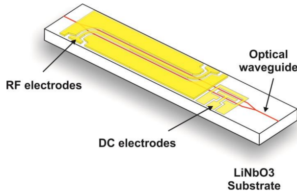
Figure 2.2: Schematic view of a \text{LiNbO}_3 intensity modulator chip. From iXblue [12]
