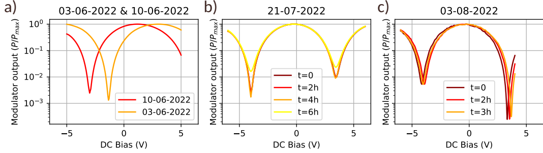
Figure 4.2: The transfer function of the EOM, plotted in log scale, measured over the course of 2 months. Figure (a) shows a significant change of the transfer function. Figure (b) shows a day where the transfer function was extremely stable in the span of 6 hours. Figure (c) shows a day where the transfer function drifted significantly in the span of 3 hours.
