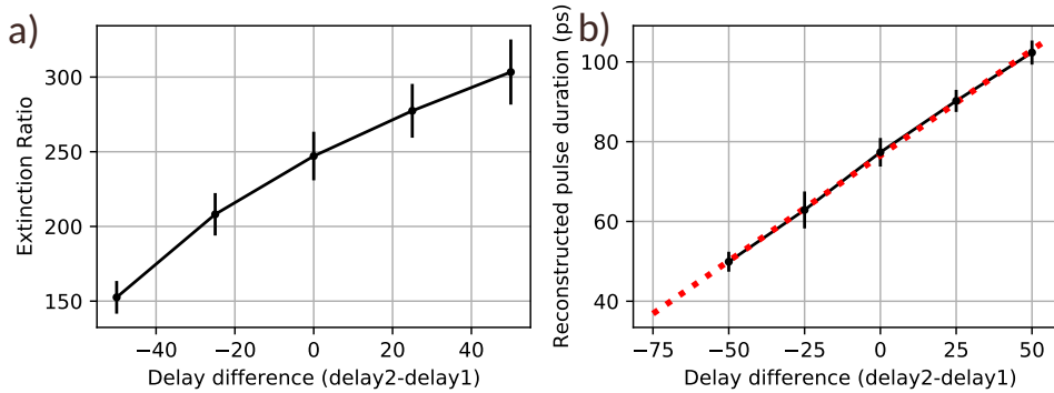
Figure 4.13: (a) Averaged extinction ratio and (b) reconstructed pulse duration as function of delay difference. The red dotted line shows a linear fit of (0.53 \pm 0.01)x + (76.5 \pm 0.3)\text{ps} .
