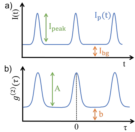
Figure 4.4: Drawing showing the definitions of the different parameters in (a) time domain and (b) g^{(2)}(\tau) .
