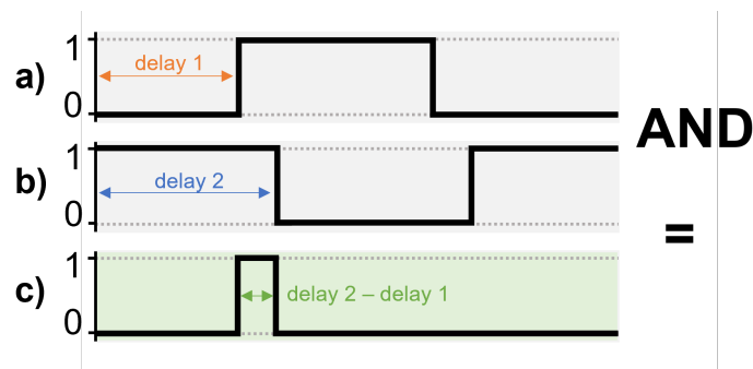
Figure 2.4: Schematic of how the short pulses are created in the Pulse compressor. Figure (a) shows the long pulse in delay line 1, (b) shows the inverted long pulse in delay line 2 and (c) shows the resulting short pulse after the AND gate.
