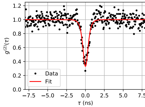
Figure 5.2: Result of a CW HBT measurement of the QD light, for 3.2 nW. The fit shows a dip of 0.34 \pm 0.02 .
