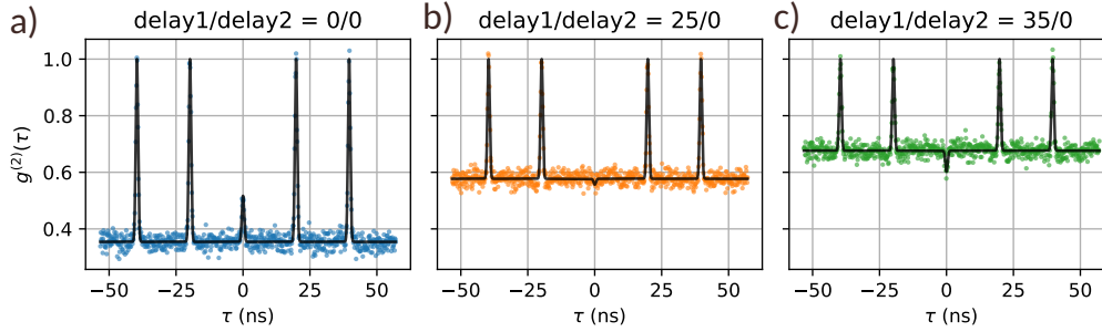
Figure 5.5: Measurements of g^{(2)}(\tau) for pulsed excitation. Data taken on 21-07-2022, for three different pulse durations. (a) has (\text{delay1}, \text{delay2}) = (0 \text{ ps}, 0 \text{ ps}) , (b) has shorter pulses of (25 \text{ ps}, 0 \text{ ps}) , and (c) even shorter pulses of (35 \text{ ps}, 0 \text{ ps}) .
