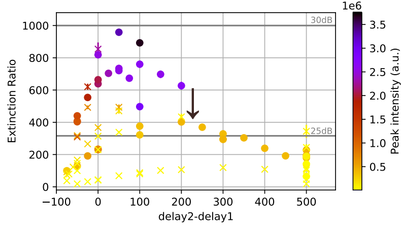
Figure 4.8: The reconstructed extinction ratios for different pulse durations and different laser powers. The color indicates an estimate of the intensity at the peaks of the pulses. The dots represent HBT measurements and the crosses TCSPC measurements (Sec. 4.5). The arrow indicates a decrease of a factor \sim 10 in optical power.
