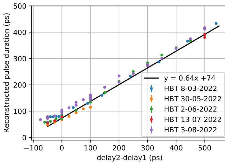
Figure I.1: The reconstructed pulse durations for Gaussian pulse assumptions. The colors indicate data taken at different dates. The solid black line indicates a linear fit through the Gaussian-ansatz data. The purple data was measured in the positive DC bias minimum, which showed significant drifting during the measurements. Because of this, it was decided not to include this data in the main text, and limit the study to the more stable negative bias minimum.
