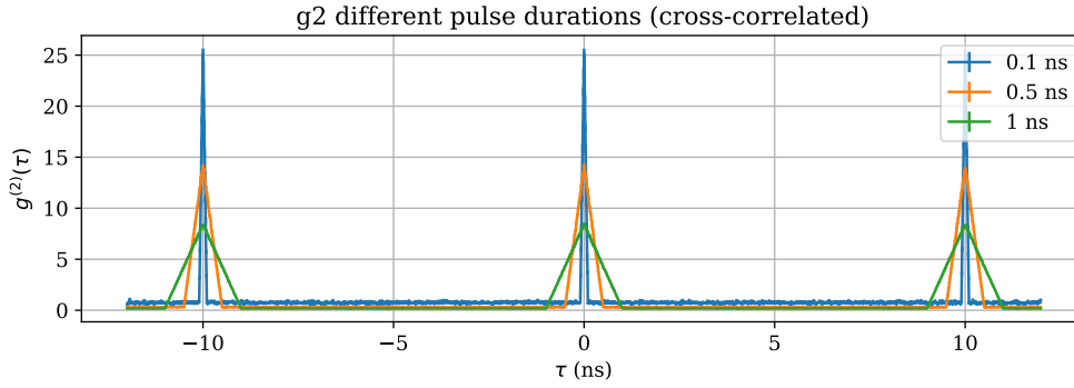
Figure 3.2: Simulation for three block pulses of different durations, simulated for 1 ms with a period of 10 ns, an intensity of 10^{10} photons/sec, 1% background light and perfect detectors.
