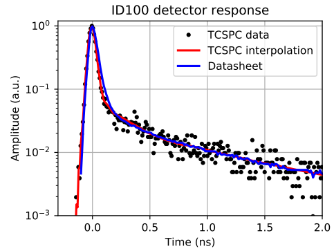
Figure 4.3: Interpolations of the timing response of the ID100 SPADs. The y-axis shows normalized counts on a log scale and the x-axis time in ns, where the peaks are shifted to t=0 . The blue line the extracted data from the ID100 datasheet and the red line shows the TCSPC measurement interpolation.
