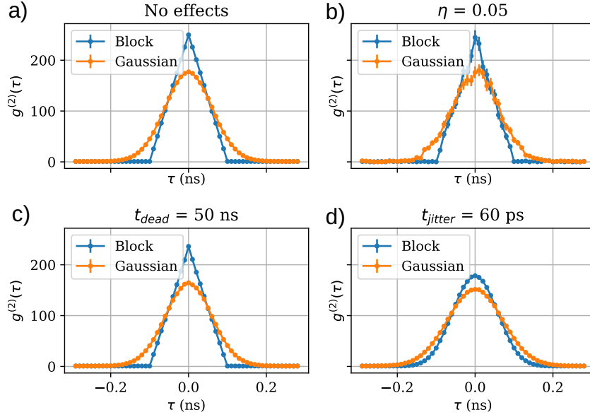
Figure 3.3: Simulation of different detector effects for block pulses and Gaussian pulses. The pulses were simulated for 0.5 s with a pulse duration of 100 ps, a period of 100 ns, an intensity of 10^{10} photons/sec and 0.1% background light.
