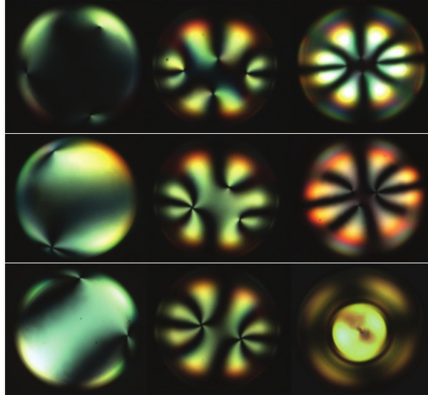
The first row shows different configurations of a nematic shell with four defects of charge \frac{1}{2} . The second row shows different configurations of a nematic shell with three defects (one with charge 1 and two with \frac{1}{2} ). The last row shows different configurations of a nematic shell with two defects of charge 1.
