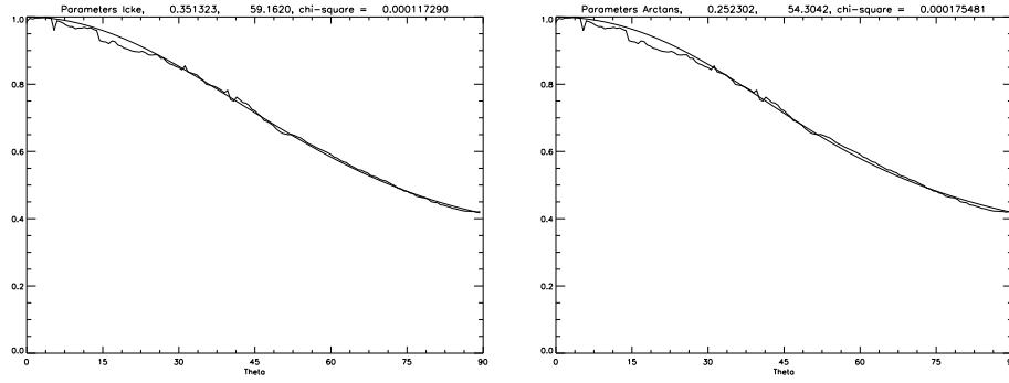
Figure 4.6: \chi -square fits for the normalized density function of the Hourglass nebula with function (4.53) at the left and function (4.54) at the right. Left: \mu = 0.3513 , \sigma = 59.16^\circ and \chi^2 = 0.00012 . Right: \delta = 0.2523 , \sigma = 54.30^\circ and \chi^2 = 0.00018 .
