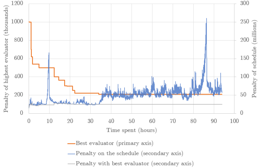
Figure 20: The development of the penalty on the schedule from Figure 13 during phase two.
