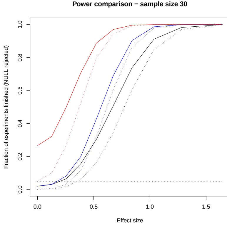
Figure 7.1: A comparison of the rejection rate (power) as the effect size increases. The Student's t-test is red, the median martingale test is black, and the Jeffreys Bayesian t-test is blue. The solid lines use optional stopping. The dotted lines do not. The threshold Bayes factor equals 20. The horizontal dotted line indicates a five percent false positive rate. The data points are normally distributed.
