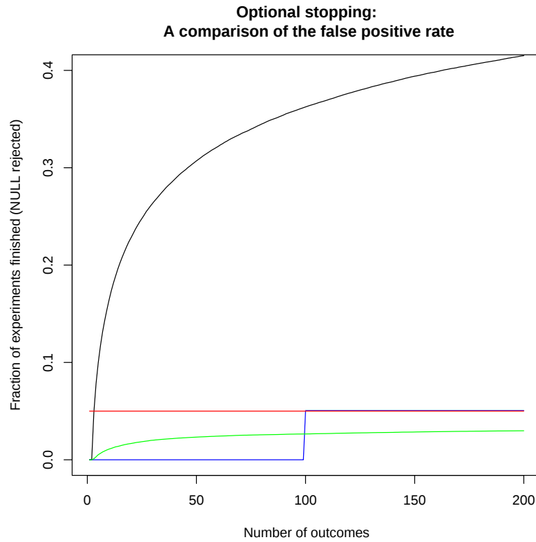
Figure 9.1: A comparison of the false positive rate as the sample size increases. The Student's t-test with optional stopping is black, the Jeffreys Bayesian t-test (with optional stopping) is green, and the Student's t-test stopping after 100 outcomes is blue. The horizontal red line indicates a five percent false positive rate. The data points are N(0, 1) -distributed.
