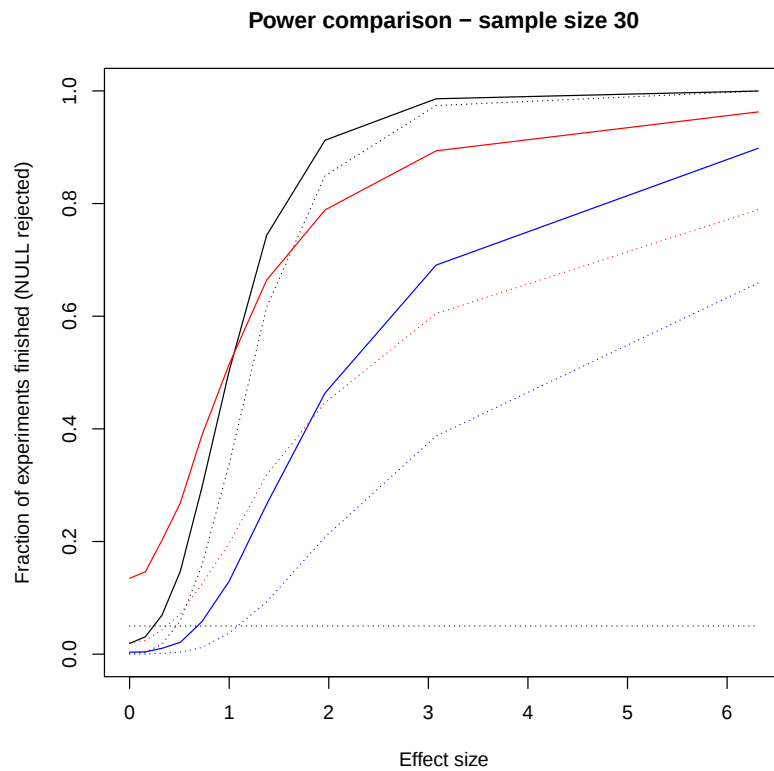
Figure 7.2: A comparison of the rejection rate (power) as the effect size increases. The Student's t-test is red, the median martingale test is black, and the Jeffreys Bayesian t-test is blue. The solid lines use optional stopping. The dotted lines do not. The threshold Bayes factor equals 20. The horizontal dotted line indicates a five percent false positive rate. The data points are Cauchy distributed.
