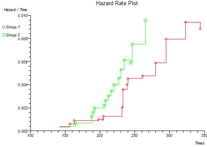
Figure 7.2: Two obligor's hazard rate plot (Source: [1])
