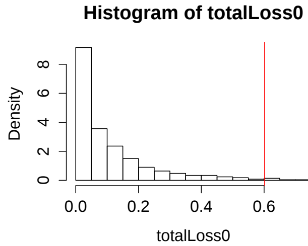
Figure 4.3: The initial portfolio losses with 99% quantile line
