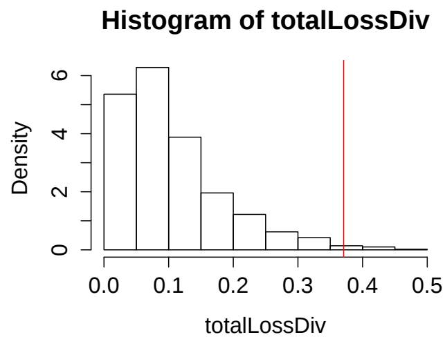
Figure 4.4: The diversified portfolio losses with 99% quantile line
