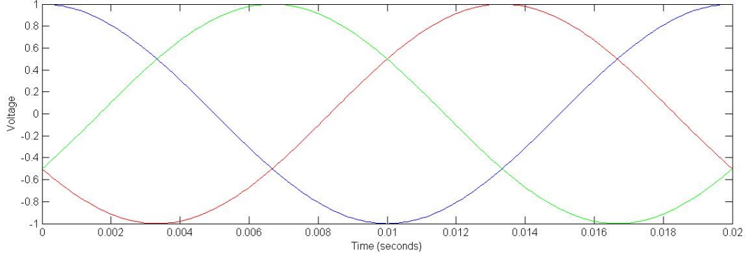
Figure 1: Voltage profile of a three phase power flow with V_{\max} = 1 and a frequency of 50 Hz. The blue line has no phase shift, the green line is shifted 120 degrees and the red line has a 240 degrees phase shift.
