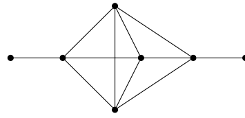
(b) Graph with \lambda_2 \approx 0.70 , R^{\text{norm}} \approx 0.28
