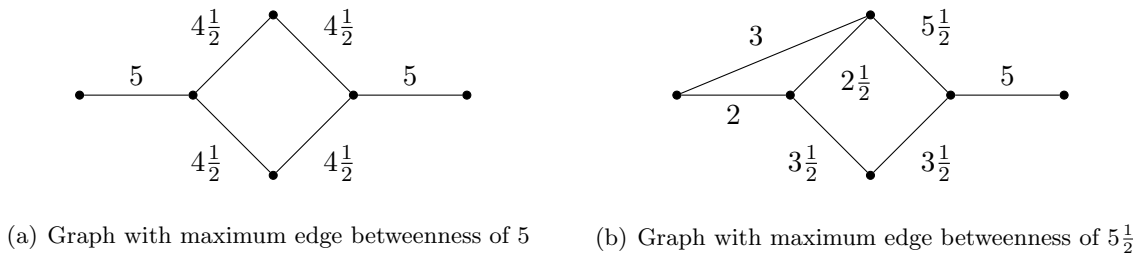
Figure 2.1. The maximum edge betweenness can increase when an edge is added. The betweenness of each edge is given in the graphs.
