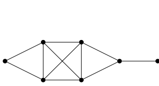
(a) Graph with \lambda_2 \approx 0.68 , R^{\text{norm}} \approx 0.30
