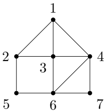
(a) Graph with R^{\text{norm}} \approx 0.403
