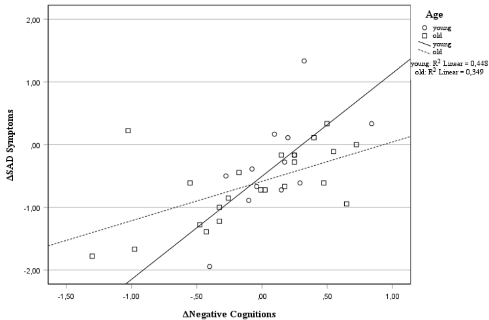
Figure 3. Scatter Plot of Moderation Analysis for Two Age Groups
