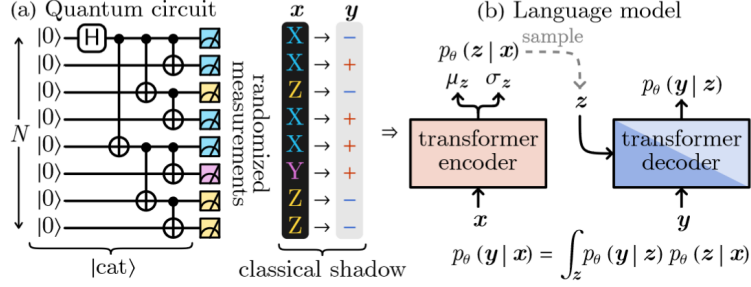
Figure 3.1: A schema for the classical shadow. The quantum Circuits were built up to prepare the quantum state (we select GHZ-state, W-state and a non-entangled state (ALL zero-state)). Randomized Pauli Measurements was applied to the pre-prepared state to generate the shadow data-set (x, y) . Then the generative model, classical shadow transformer (transformer-based \beta -VAE architecture) is trained to learn the distribution of p(y|x) . As a result, we follow the specific quantum channel M for Random Pauli Measurement to reconstruct the original state and extract related quantum information from classical data. [6]
