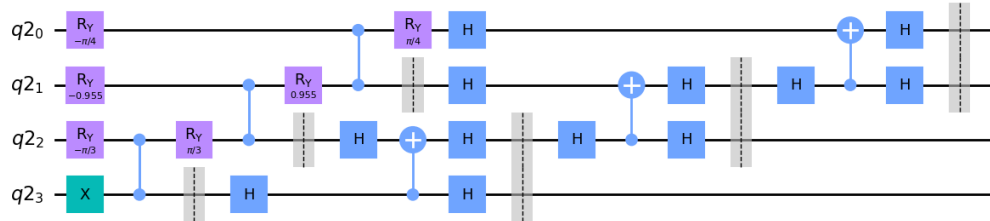
Figure 3.5: qiskit visualization for a four-qubit W state circuit
