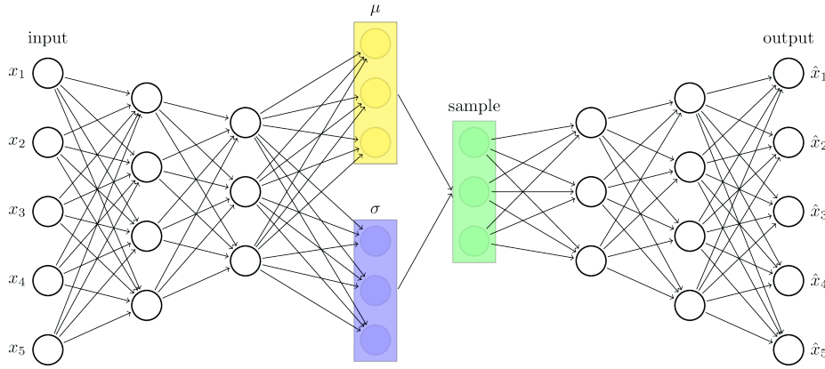
Figure 2.3: A diagrammatic representation of a Variational Autoencoder (VAE). The left section illustrates the Encoder where the input image x is compressed into a lower-dimensional latent space Z characterized by the learned mean \mu_{z|x} and standard deviation \Sigma_{z|x} . In the central section, the latent space Z serves as a bottleneck, encapsulating the essential information required for reconstruction. The right section depicts the Decoder, which reconstructs the original input into the output image \hat{x} using the sampled latent variables. The entire process aims to minimize a composite loss function comprised of Reconstruction Loss and the Kullback-Leibler (KL) Divergence, ensuring a balance between accurate reconstruction and a well-formed latent distribution.
