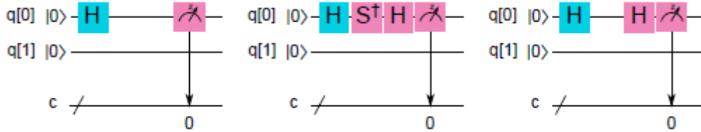
Figure 3.6: Quantum circuit used to transform Pauli Basis to Z basis. The order from left to right is corresponding to Pauli X, Y, Z. The plot is cited from "Quantum Algorithm Implementations for Beginners"[27]
