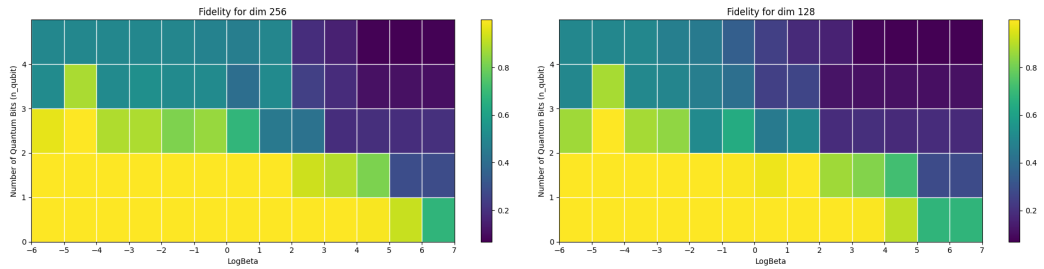
Figure 4.6: Fidelity heatmap for reconstructed ghz -state from CST in higher latent dimension (the left one is 256 and the right one is 128)
