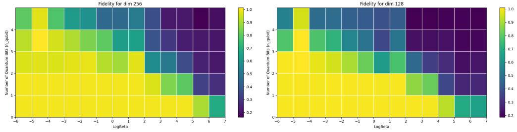
Figure 4.5: Fidelity heatmap for reconstructed W -state from CST in higher latent dimension (the left one is 256 and the right one is 128)
