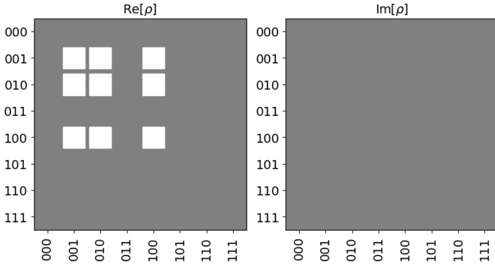
Figure 4.10: Density Matrix Structure for a 3-qubit w-state
