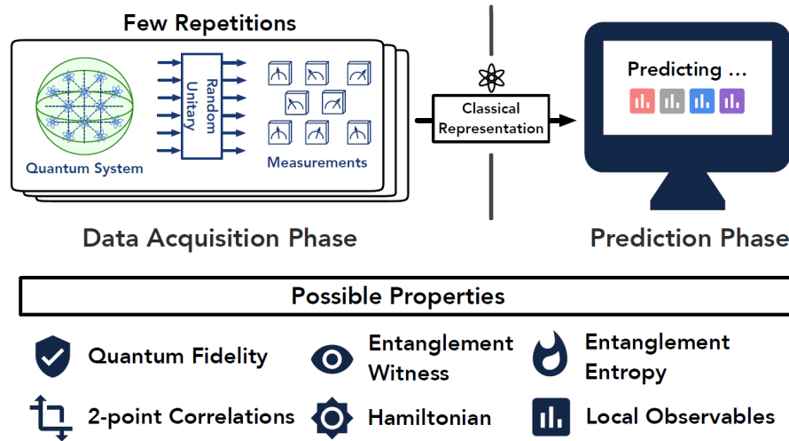
Figure 2.2: A figure from[4] that represents the procedure of shadow tomography which means predicting the properties of a quantum system from randomized measurements. First, we apply a set of Unitary transformations and random measurements on copies of a n -qubit system to obtain the classical shadow data set. Then we get the prediction of the system using median-of-means protocol on these datasets
