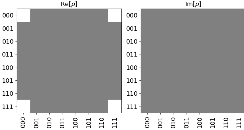
Figure 4.9: Density Matrix Structure for a 3-qubit ghz-state
