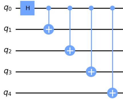
Figure 3.2: An example diagram for a 5-qubit GHZ-state Circuit
