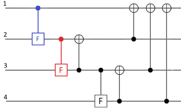
Figure 3.4: The circuit used for creating a four-qubit W state.
