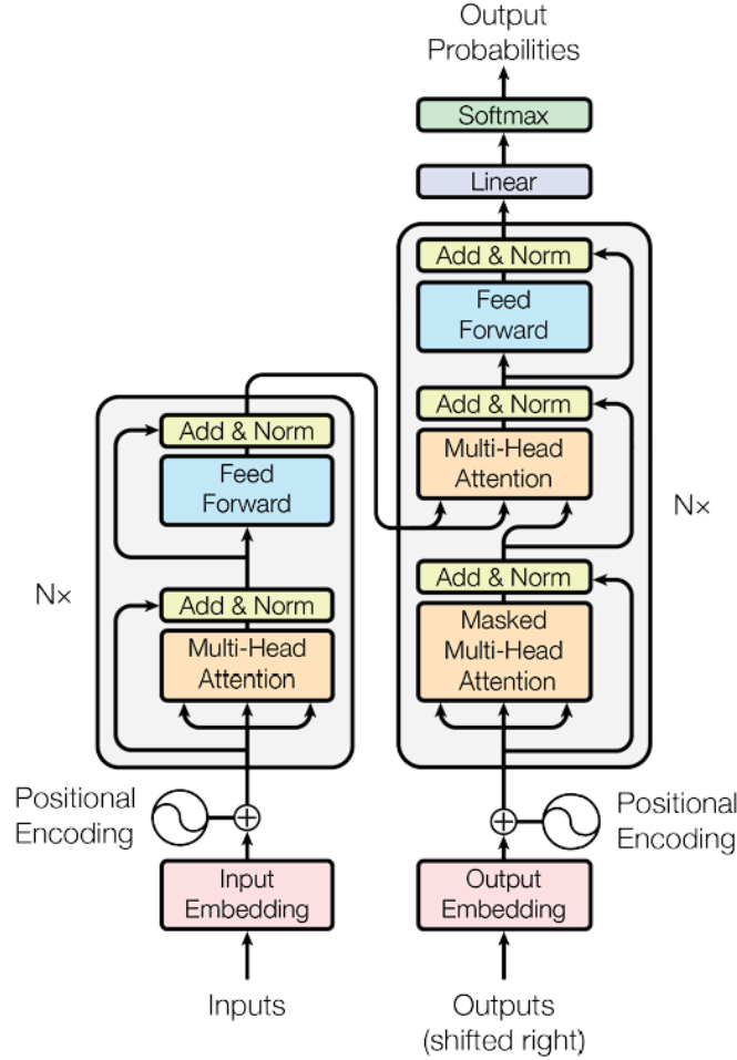
Figure 2.4: The Transformer architecture as implemented in our model. The encoder processes the input sequence in parallel, while the decoder synthesizes the output sequence, both employing self-attention and feedforward layers.
