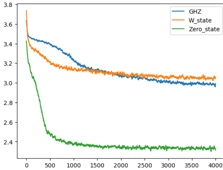
Figure 4.2: The loss history for 3 states in all 4000 training epochs, the model parameters: n\text{-qubits} = 4 , \log \beta = -6 , \dim for latent space = 64, we apply the Moving Average Filter to the curve and window\_size = 15
