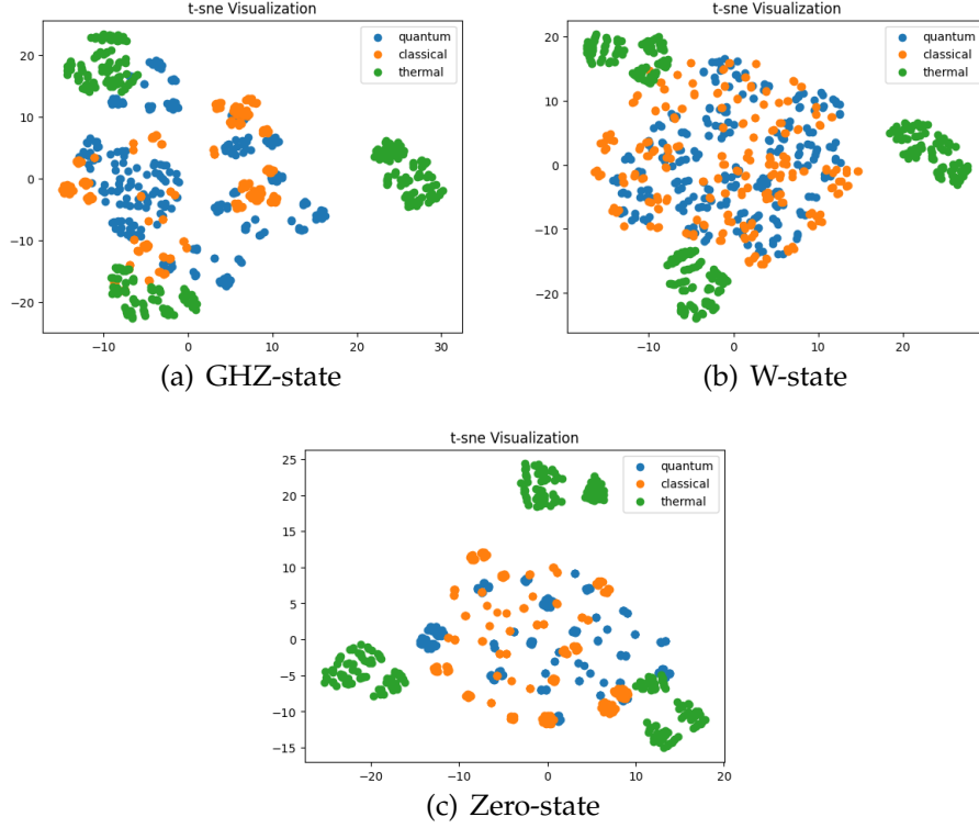
Figure 4.7: T-sne plot of the latent space of all possible observables for CST trained on different states, each dot represents a Pauli sequence and model with different information bottleneck are labelled in a different colour of Green(thermal, \log_2 \beta = 6 ), Orange(classical, \log_2 \beta = -1 ) and Blue(quantum, \log_2 \beta = -5 ), all model is trained on a 5-qubit system and dimension of latent space is 64
