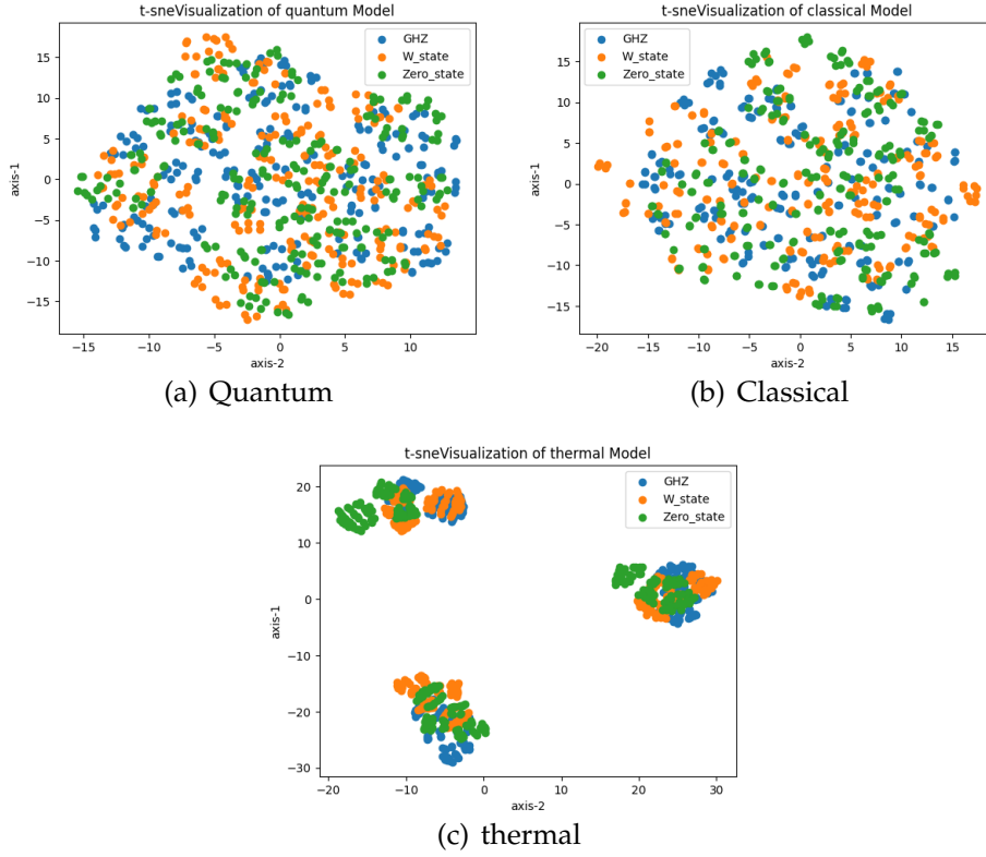
Figure 4.8: T-sne plot of the latent space of all possible observables of three states for different information bottleneck regions, each dot represents a Pauli sequence and model are labelled in different color of blue(GHZ-state). orange (W-state). and green (Zero-state), all model is trained on a 5-qubit system and the dimension of latent space is 64
