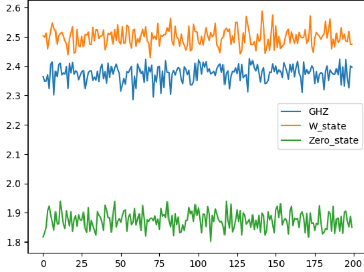
Figure 4.1: The loss history for 3 states in the last 200 training epoch, the model parameters: n\text{-qubits} = 4 , \log \beta = -6 , \dim for latent space = 64
