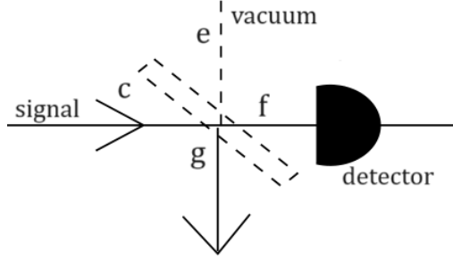
Figure 3: An inefficient photon-count detector modelled as an ideal detector preceded by a beam splitter.
