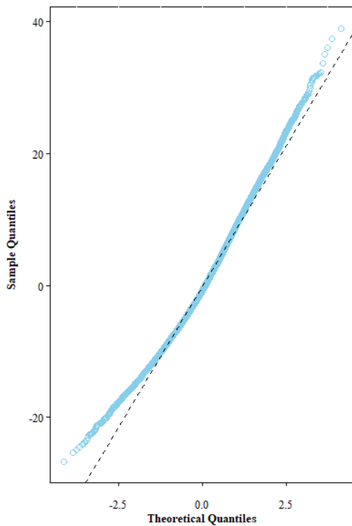
Q-Q Plot Residuals of Anxiety Scores with Personality Traits
