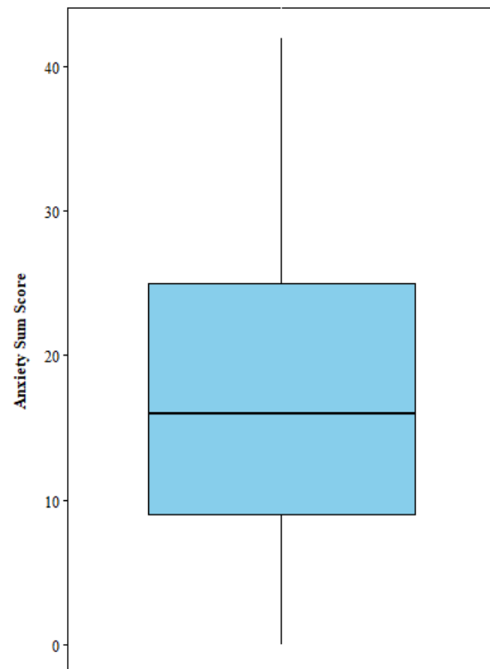
Boxplot of Total Anxiety Scores
