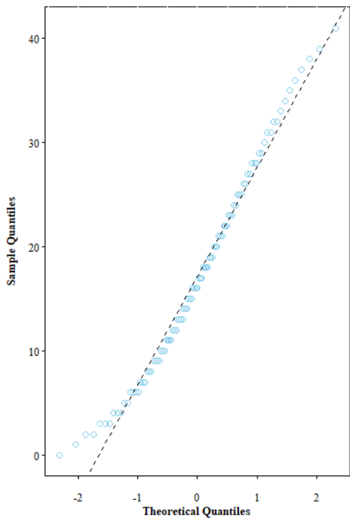
Q-Q Plot of Total Anxiety Scores
