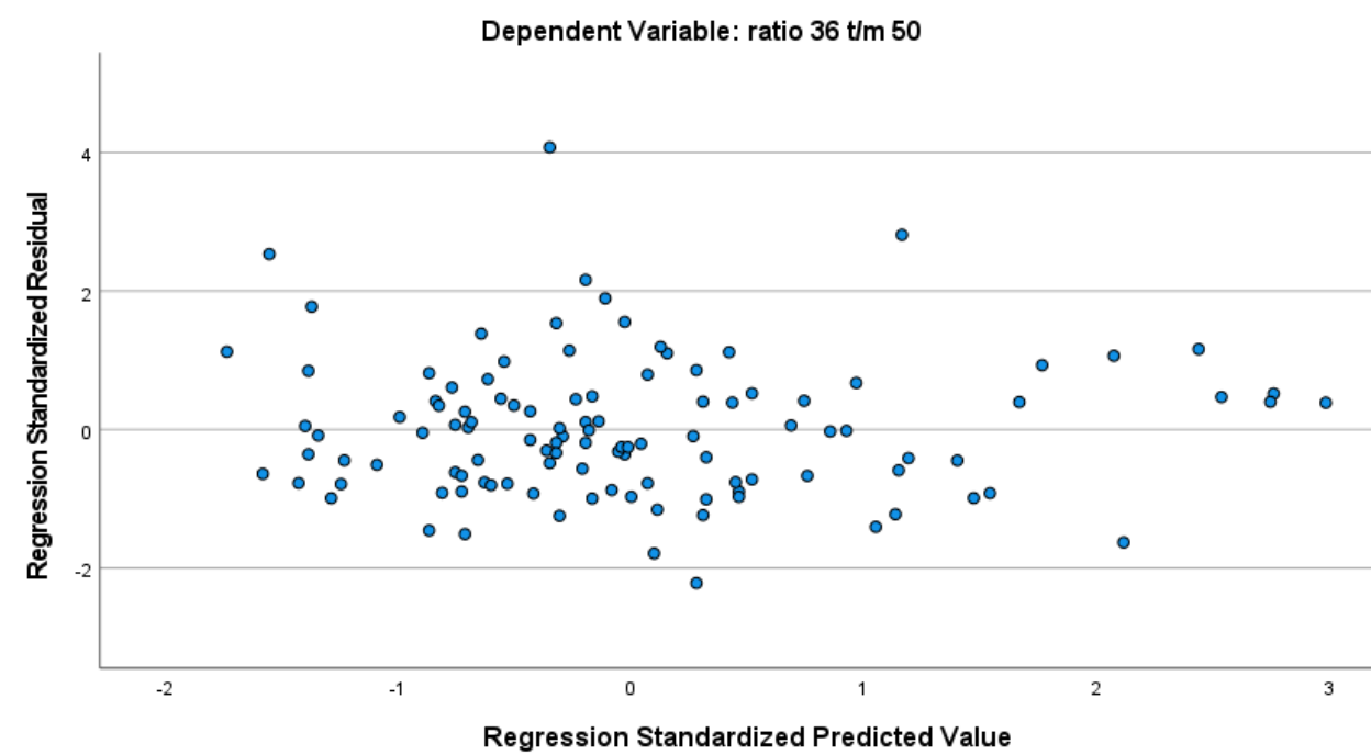
Scatterplot
