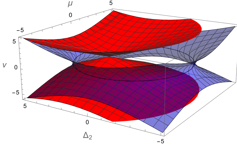
Figure 10.2: The level set of \det(\mathcal{H}_{SC2}(0)) = 0 , in red, and the level set of \det(\mathcal{H}_{SC2}(\pm\pi/2)) = 0 , in blue, for t = 2\Delta_1 normalised by \Delta_1 by substituting t = 2 and \Delta_1 = 1 in Eq. 10.16 and Eq. 10.17 respectively. This is a part of the critical manifold of the superconducting equivalent of the Rice-Mele model.
