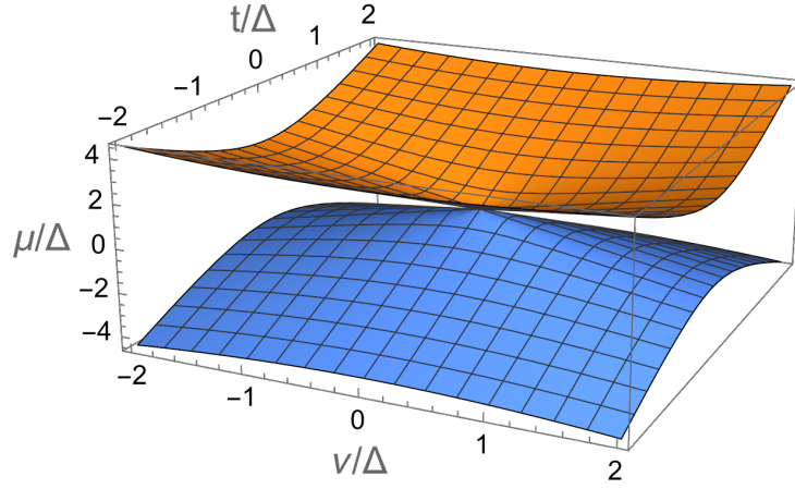
Figure 9.8: The level set of \det(\mathcal{H}_{\text{Stag.Chem}}(0)) = 0 normalised by \Delta by substituting \Delta = 1 in Eq. 9.17. This is a part of the critical manifold of the superconducting chain with staggering chemical potential.
