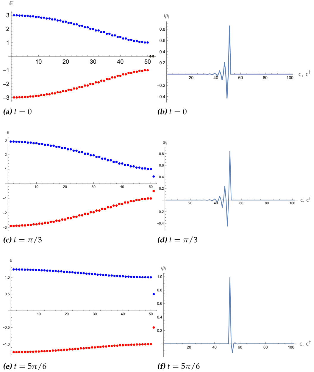
Figure 9.12: (a),(c),(e) The spectrum of a Rice-Mele model with 51 sites performing a loop described by Eq. 9.59 at t = 0 , t = \pi/3 , and t = 5\pi/6 respectively. The spectra show how throughout the loop the energies of the edge states are lifted to the bulk and brought back. (b),(d),(f) The positive energy edge state corresponding to the spectra. The x-axis depicts the Nambu spinor, Eq. 7.31, and the y-axis the coefficients such that (\psi_1, \dots, \psi_{2N})(c_1, \dots, c_N, c_1^\dagger, \dots, c_N^\dagger)^T is a normalised state.
