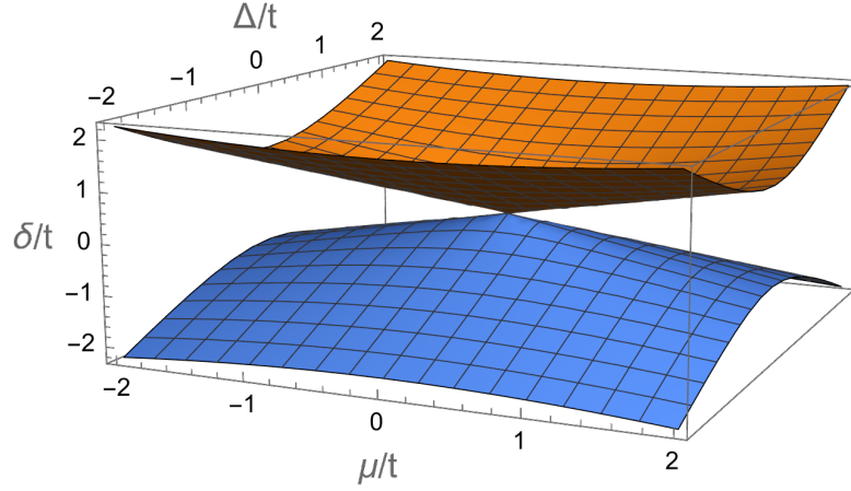
Figure 9.1: The level set of \det(\mathcal{H}_{\text{SSH}+\text{sc}}(\pm\pi/2)) = 0 normalised by t by substituting t = 1 in Eq. 9.17. This is a part of the critical manifold of the superconducting SSH-model.
