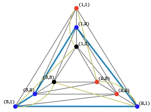
(b) Colouring of H_t(3,3)
