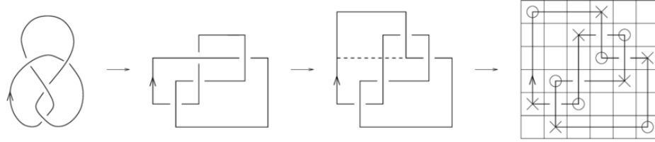
Figure 5: Transformation of a projection of the figure eight knot to a planar grid diagram
