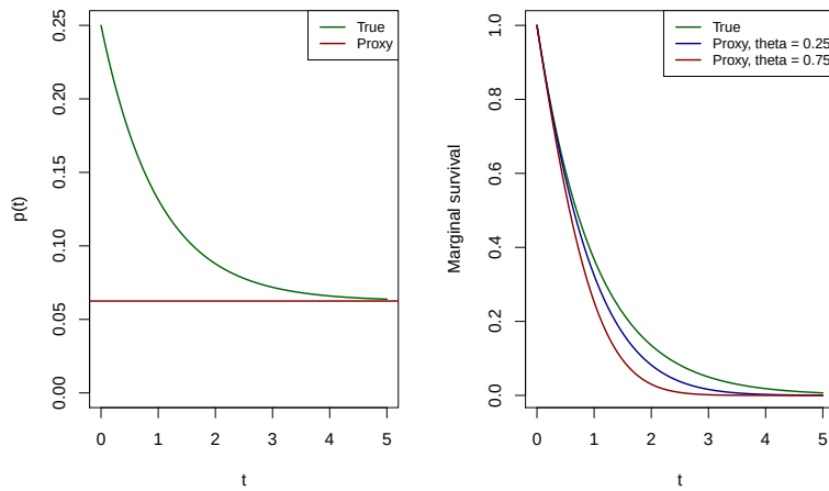
Figure 3.1: Plot of the function p(t) and the different marginal survival functions ( \theta = 0.25, 0.75 ).
