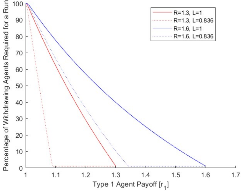
Figure 5: Smoothed Averages
