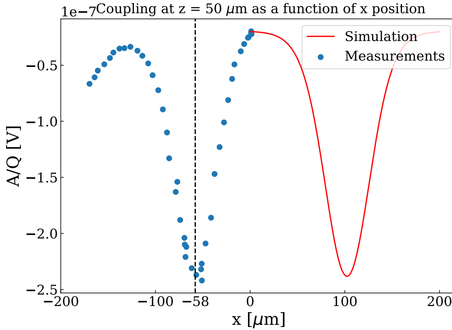
Figure 4.4: Coupling as a function of x -position. The blue dots represent the measured A/Q , the red line represents the simulation of the cantilever coupling at a height of 50\ \mu\text{m} above the sample. On the x -axis is the x -position in \mu\text{m} . On the y -axis is A/Q in \text{V} . A scaling factor was added to the simulation so that its amplitude is similar to that of the measured curve. We see that the curves have the same shape, but lie 158\ \mu\text{m} from each other.
