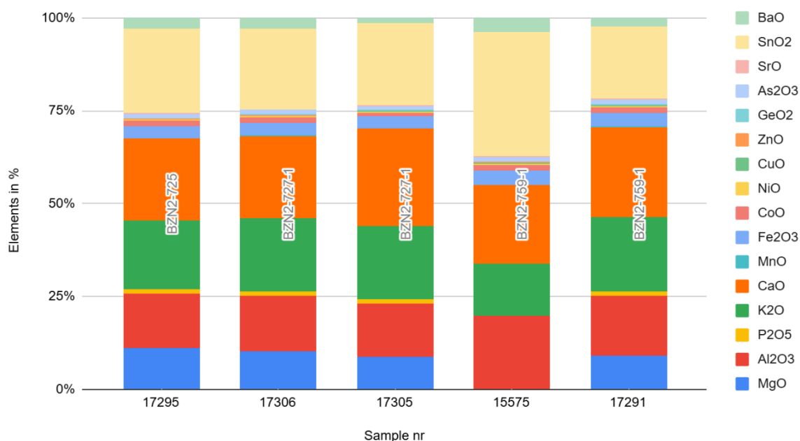
Glaze composition coat of arms without SiO 2 and PbO
