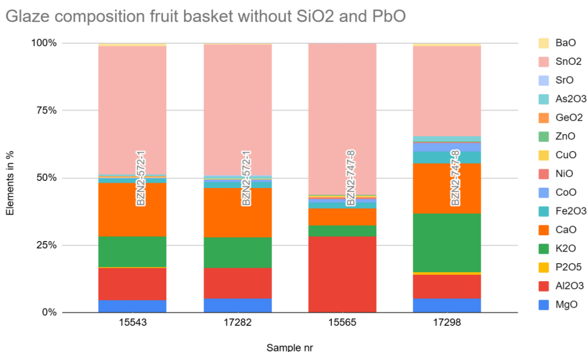
Figure 26. The composition of the glaze from the fruit basket decoration without SiO 2 and PbO.
