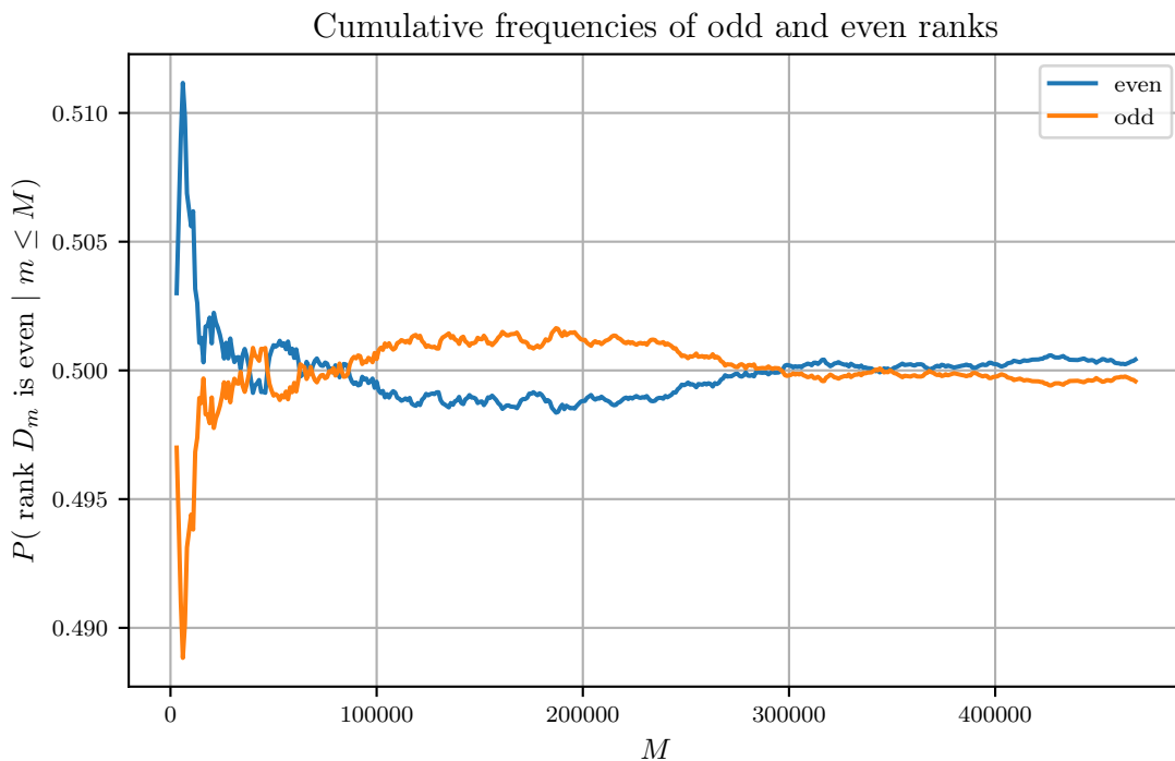
Figure 2.2: This figure shows the graphs for P(D_m \text{ is odd/even} \mid m \leq M) within our dataset. As expected, both graphs (which by definition sum to 1) seem to tend to \frac{1}{2} .
