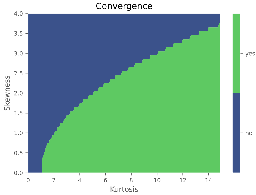
Figure 3.6: A contour plot showing the convergence of Algorithm 2 with varying skewness \gamma_1 and kurtosis \gamma_2' . The constraints were f(x) = (x, x^2, x^3, x^4) and F = (0, 1, \gamma_1, \gamma_2') , with support [-20, 20] and quadrature number n = 200 . This is a recreation of Figure 1 in [5].
