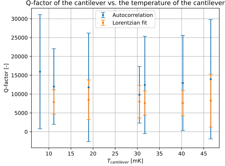
Figure 5.7: Average Q -factor of the cantilever obtained from the Lorentzian fit and autocorrelation during the analyzed periods during the discrete energy steps. The Q -factor of the period during the lowest temperature obtained from the Lorentzian fit is missing, as there was no fit data of that period available.
