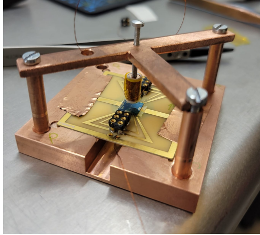
Figure 3.7: Photo of the complete sample holder
