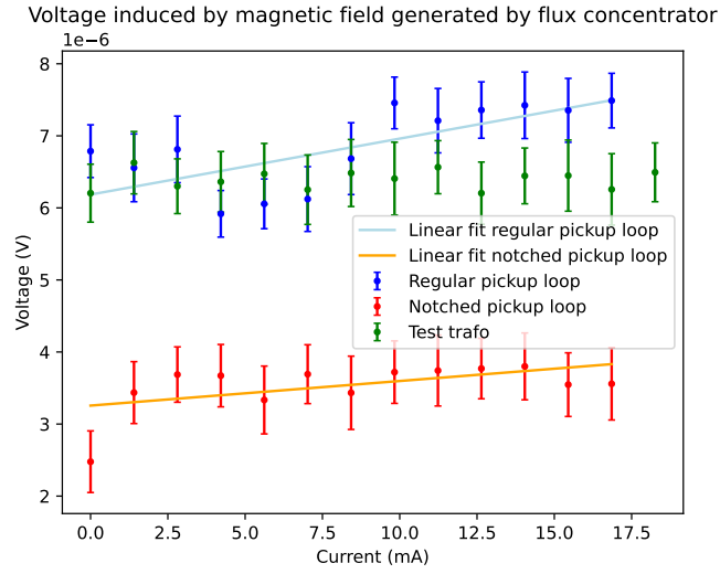
(a) Fit data regular loop: V = 7.77 \cdot 10^{-8} \cdot I + 6.18 \cdot 10^{-6} , fit data notched loop: V = 3.41 \cdot 10^{-8} \cdot I + 3.26 \cdot 10^{-6}
