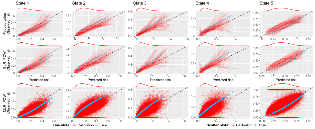
Figure 5.16: Moderate calibration plots for miscalibrated predicted calibration probabilities \hat{p}_{k,miscal2}^i , under RC scenario and sample size n = 700 .
