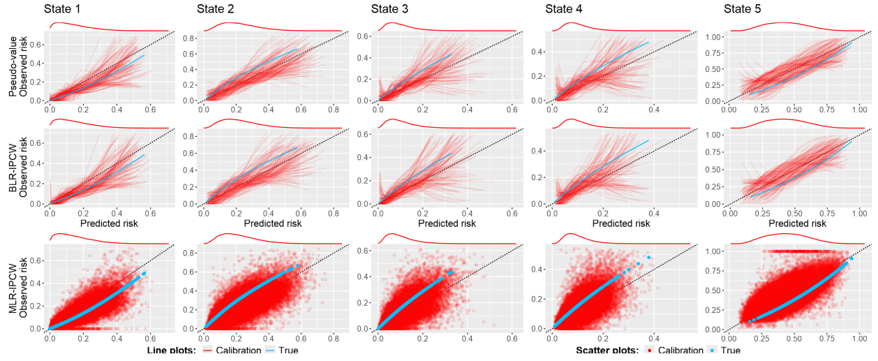
Figure 5.10: Moderate calibration plots for miscalibrated predicted calibration probabilities \hat{p}_{k,miscal2}^i , under WAC scenario and sample size n = 500 .
