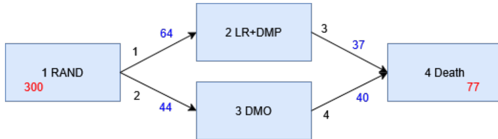
Figure 6.4: Observed state transitions in the development set with 300 patients for the 4-state model with states \{1 \text{ RAND}; 2 \text{ LR+DMP}; 3 \text{ DMO}; 4 \text{ Death}\} , in which all patients start in the randomization state. State and transition number are written in black, number of transitions in blue and number of patients starting at time of randomization and entering the death state in red.
