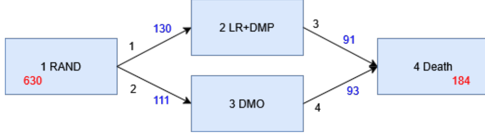
Figure 6.3: Multi-state model with 4 states \{1 \text{ RAND: randomization}; 2 \text{ LR+DMP: local recurrence and distant pulmonary metastasis}; 3 \text{ DMO: other distant metastasis}; 4 \text{ Death}\} and all patients starting in the randomization state. State and transition number are written in black, number of transitions in blue and number of patients starting at time of randomization and entering the death state in red.
