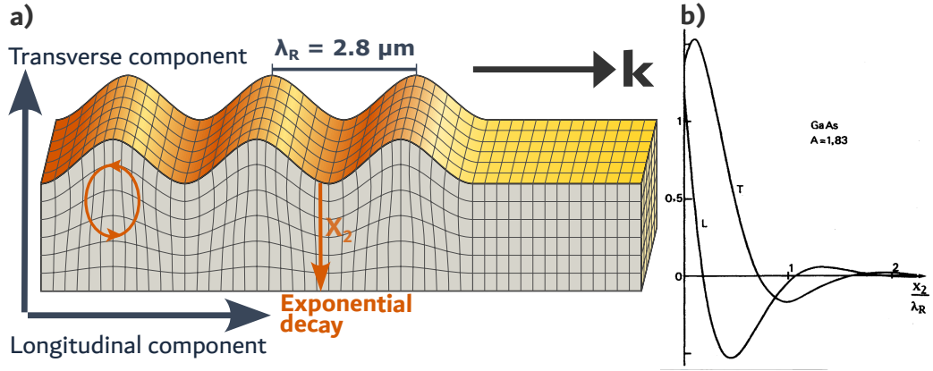
Figure 2.1: a) Rayleigh wave. The transverse (T) and longitudinal (L) component add up to a elliptical movement of atoms and decay into the bulk. \lambda_R is the SAW wavelength in GaAs and \mathbf{k} indicates the direction of propagation [1]. b) Change of displacement into the bulk of the SAW components in (010)-cut GaAs. x_2 is the distance into the bulk. A is the anisotropy factor as defined by Royer and Dieulesaint [2].
